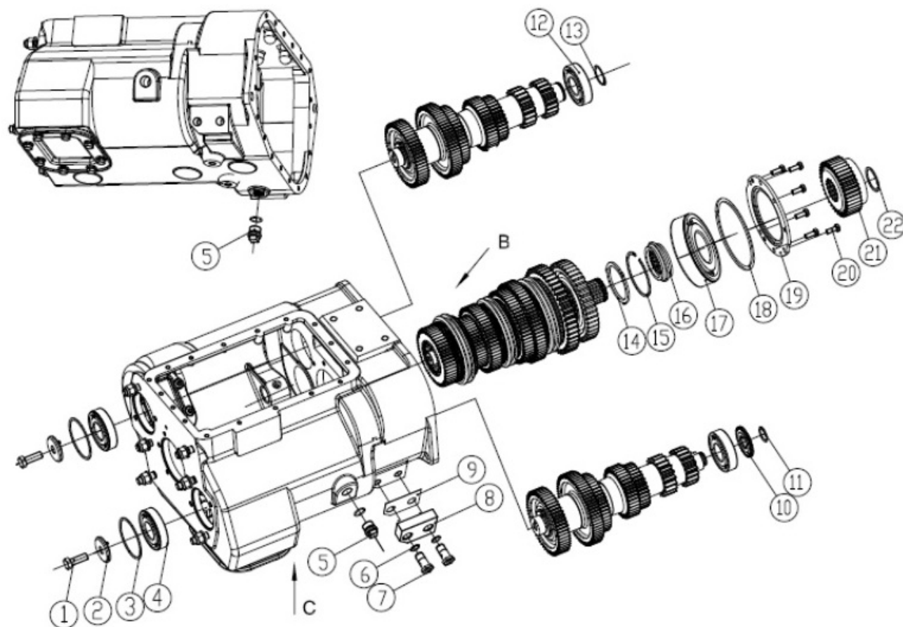
VIEW C
